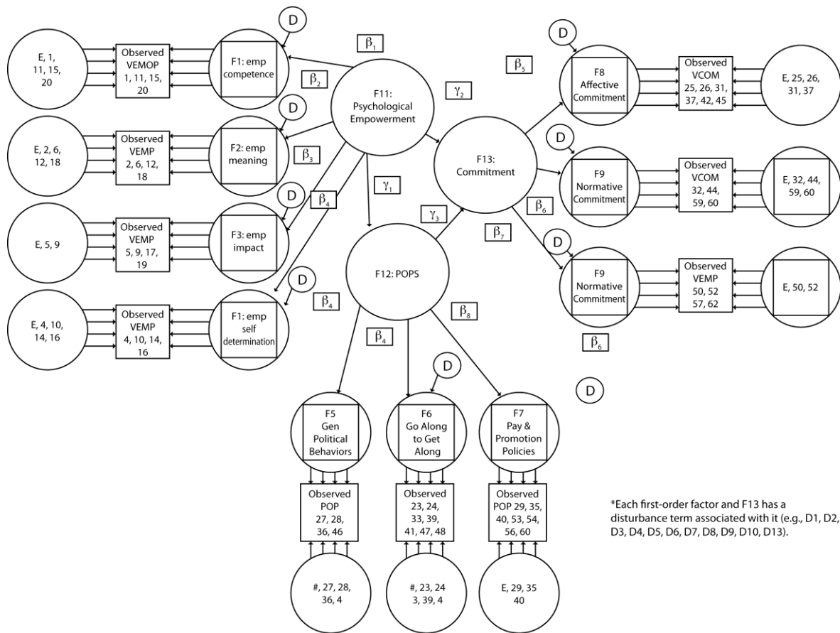
Figure 1: Full Structural Equation Model with EQS Notation
